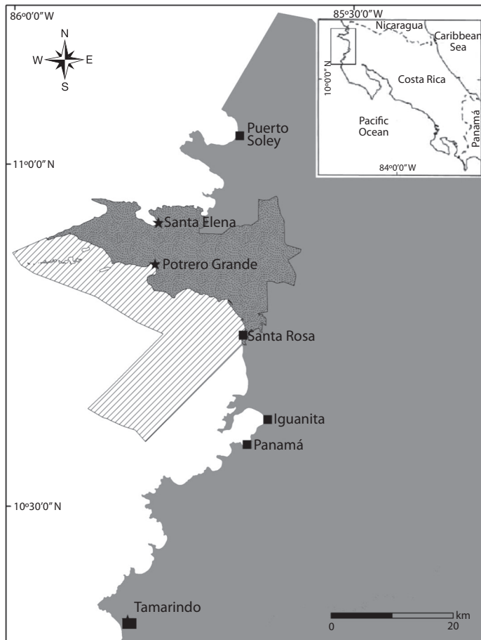
Fig. 1. North Pacific mangrove study sites Potrero Grande and Santa Elena (stars) within Santa Rosa National Par (dark grey with pattern) and adjacent marine protected area (white with stripes). Previous studies (squares) Santa Rosa (Pool et al., 1977); Puerto Soley (Soto & Jiménez, 1982); Iguanita and Playa Panamá (Samper-Villarreal et al., 2012).
