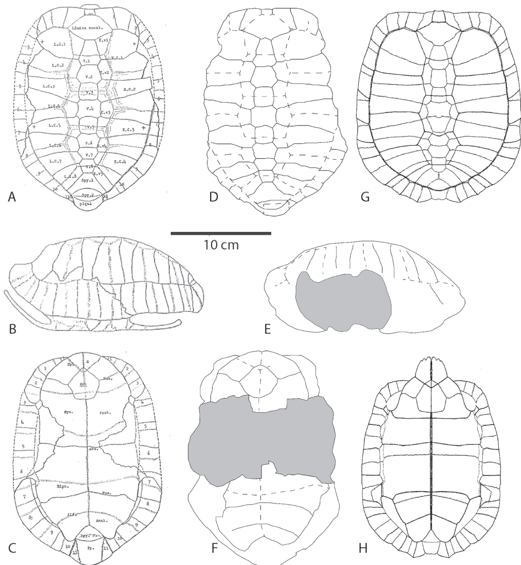
Fig.1: Geochelone costarricensis A-C, original reconstruction from Segura (1944); D-F, revised reconstructions. G-H, reconstruction of Oligopherus laticunea based on Hutchison (1996) A, D, G, dorsal view; B, E, lateral view; C, F, H, ventral view. Abbreviations: Anal, anal scute; Abd, Abdominal scute; fem, Femoral scute; Epi, epiplastron; Ent, entoplastron; G, gular scute; Hum, humeral scute; Hipo, hypoplastron; Hyo, hyoplastron; L.C., Left Costal; V., neural; Pect, pectoral scute; Py, pygal; Spy, suprapygal; E.C., right costal; Xic, xiplastron.
