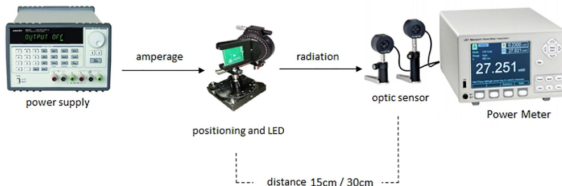
Figure 4. Schematic diagram made for measuring LED power
