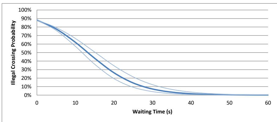
Fig. 7. Illegal crossing probability versus pedestrian waiting time
