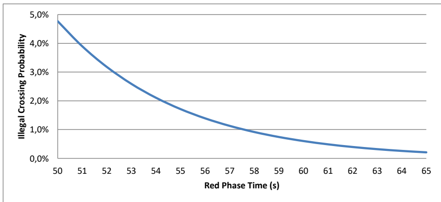
Fig. 6. Illegal crossing probability versus red phase time.
