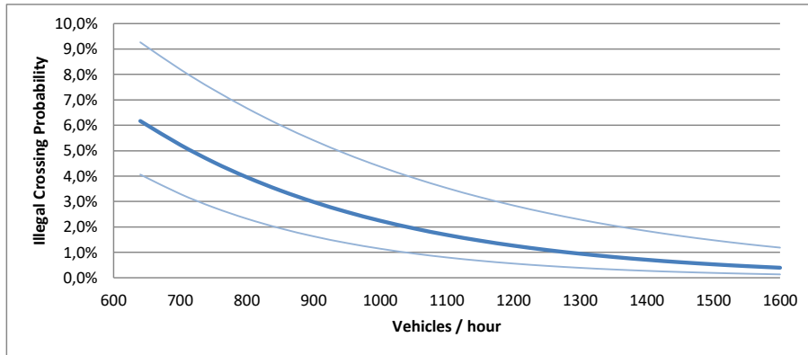
Fig. 3. Illegal crossing probability versus vehicle volume.
