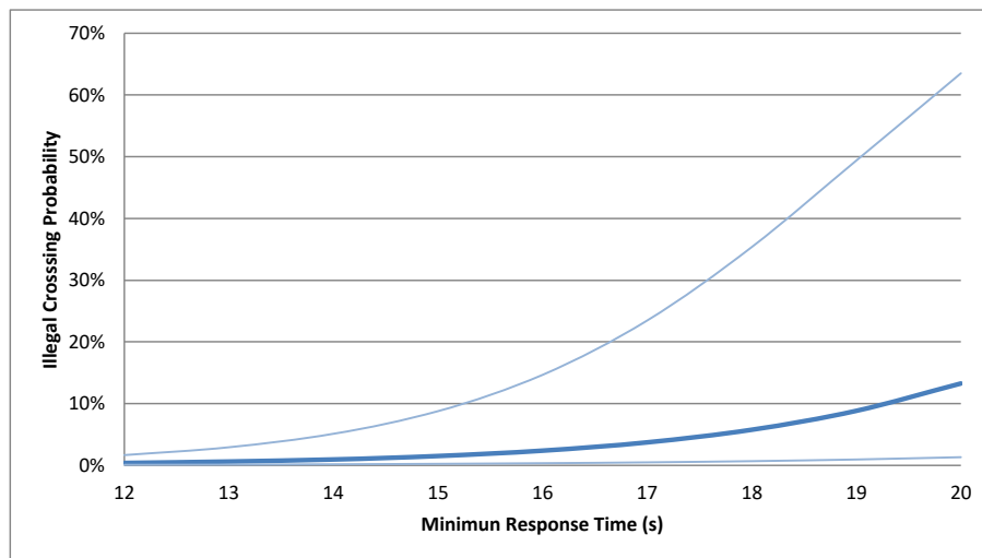
Fig. 8. Illegal crossing probability versus traffic light minimum response time.
