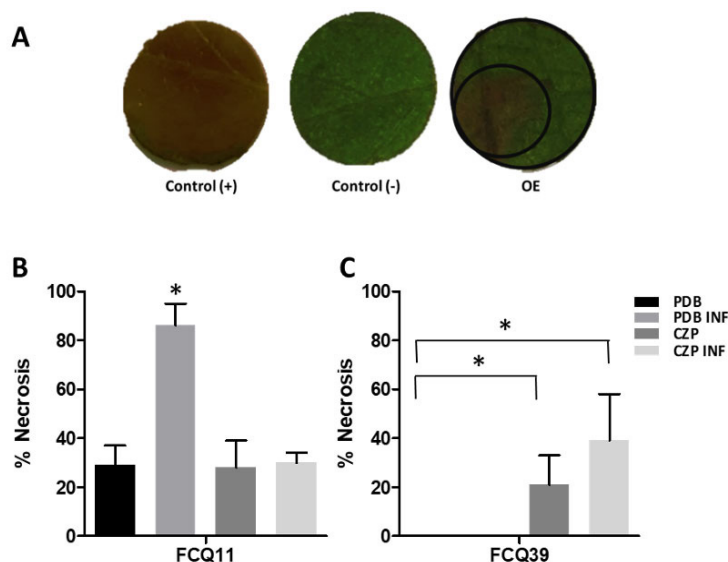
Figure 2. Phytotoxicity bioassay results. A. Representative images showing phytotoxic activity of metabolites secreted by Macrophomina phaseolina FCQ11 on soy leaves discs. Control (+): \text{H}_3\text{PO}_4 solution as positive control; Control (-): acetoneitrile as negative control; OE: crude organic extract from PDB INF tested at 50 \mu\text{g} . Departamento de Química Biológica, Facultad de Ciencias Químicas, Universidad Nacional de Asunción, Paraguay. 2016.
