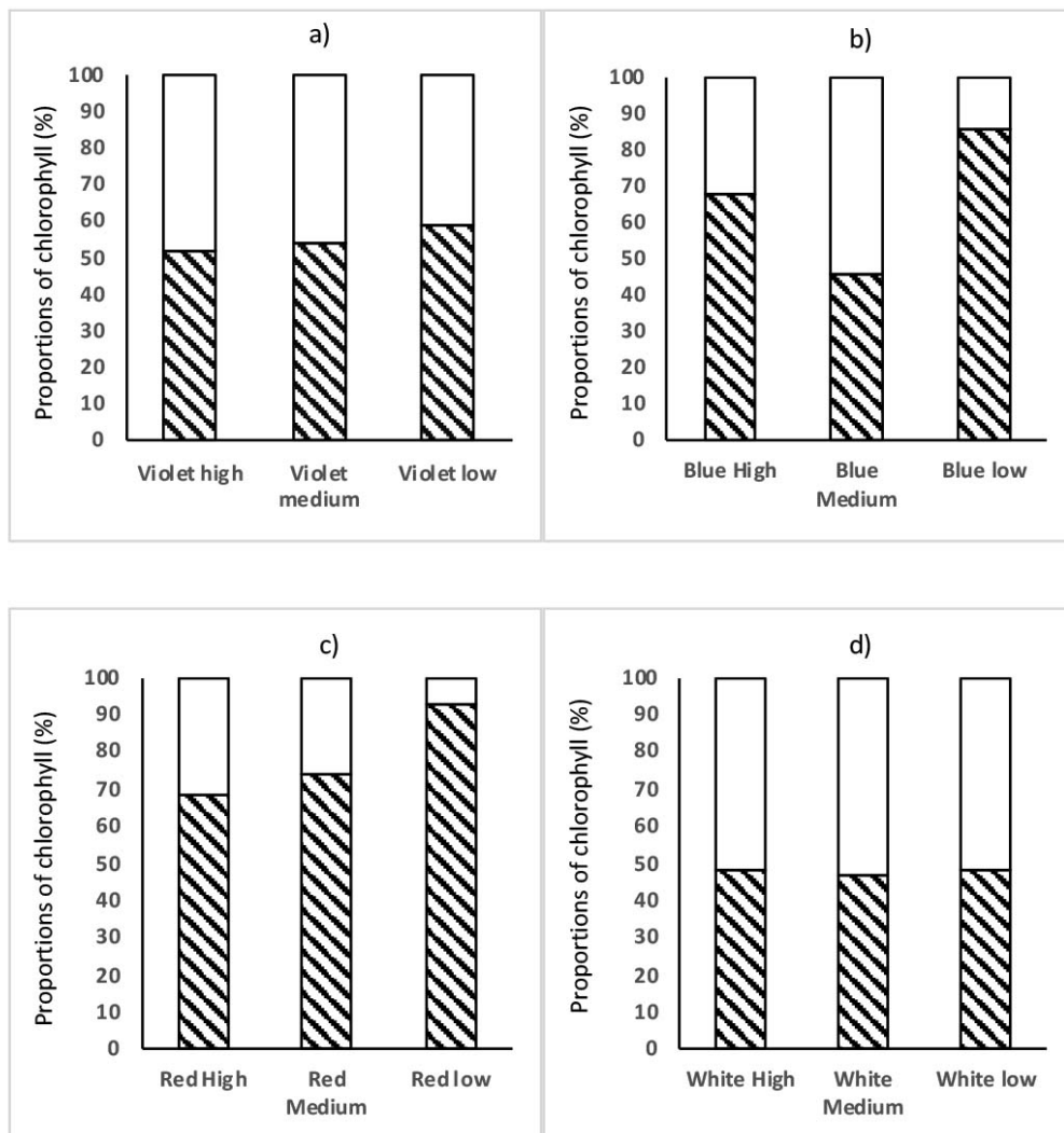
Figure 1. Proportions of chlorophyll a (■) and b (□) (%) under a) violet, b) blue, c) red, and d) white lights in strawberry ( Fragaria ananassa ) cultivar San Andreas. Laboratory of Plant Genetic, Department of Agronomy, Universidad de Guanajuato, Mexico, 2020.
