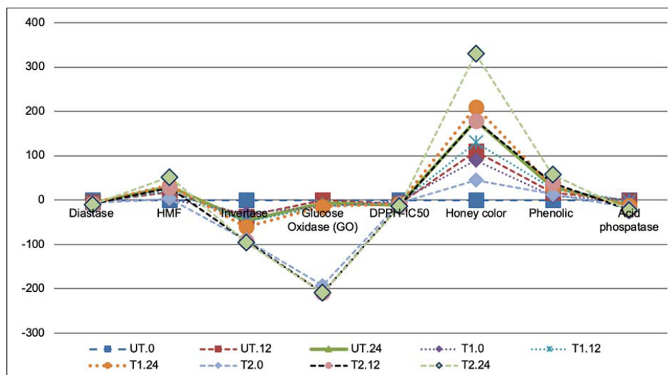
Figure 2. Physicochemical changes selected for the treatment and storage process. Standard control UT0 (unheated and not stored), UT1 (heated at 40 °C for 48 h) and UT2 (heated at 70 °C for 7 h). UT was stored for 12 months (UT12) and for 24 months (UT24). T1 was not stored (T1.0), stored for 12 months (T1.12) and for 24 months (T1.24). T2 without storage (T2.0), stored for 12 months (T2.12), and for 24 months (T2.24). Chemical engineering Department. Institute Sains and Technology Al Kamal-Jakarta, Indonesia. 2022.
