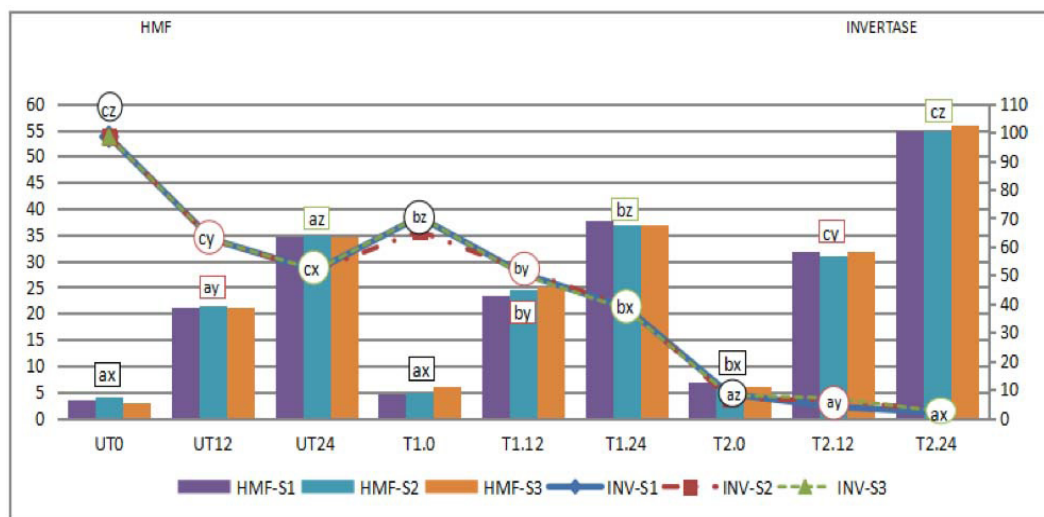
Figure 1. Effect of heating and storage on the activity of invertase and HMF in Klanceng honey. The samples of Klanceng honey (S1, S2, S3) were analyzed for their invertase (INV-S1, INV-S2, INV-S3) and HMF (HMF-S1, HMF-S2, HMF-S3) activity. The same superscript used (two letters) indicates no significant difference. Superscripts for UT, T1, and T2 were a, b, c. Superscripts used for storage times (0, 12, and 24) were x, y, z. National Innovation Research Agency Laboratory, Jakarta, Indonesia. 2022.
