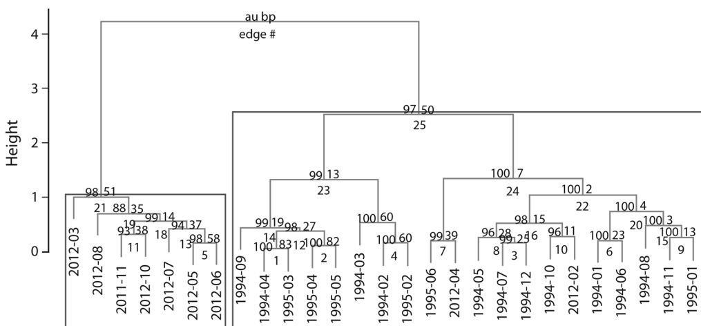
Fig. 5. Cluster dendrogram with AU (left) / BP(right) values (%) of dissimilarity between leaf-litter amphibian surveys (year and month) carried on in 1994-95 and 2011-12 in the San Lorencito River Station. Rectangles indicate clusters with AU \geq 95.
