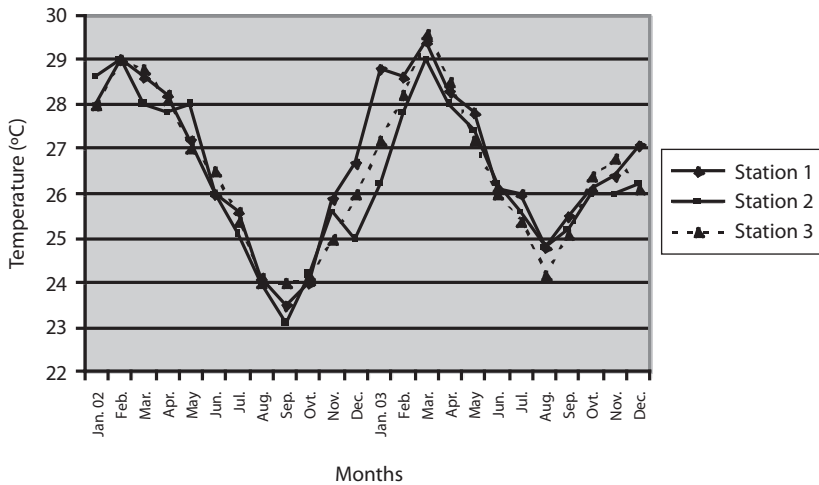
Fig. 2. Monthly mean variations in surface water temperature of Oyun Reservoir.
