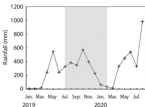
Fig. 2. Rainfall ( \text{mm month}^{-1} ) data from January 2019 through August 2020 from the Instituto Meteorológico Nacional de Costa Rica station, near Golfo Dulce ( 08^{\circ} 42' 03'' N, 83^{\circ} 30' 49'' W, at 80 m above sea level). Gray shading indicates the timeframe of the experiment.
